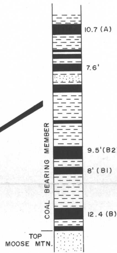
TENT MOUNTAIN V-1" = 75'
