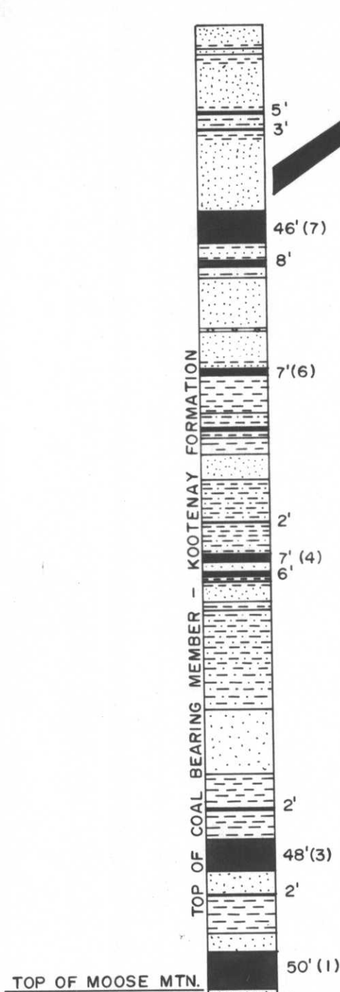
FLATHEAD RIDGE V-1" = 200'
