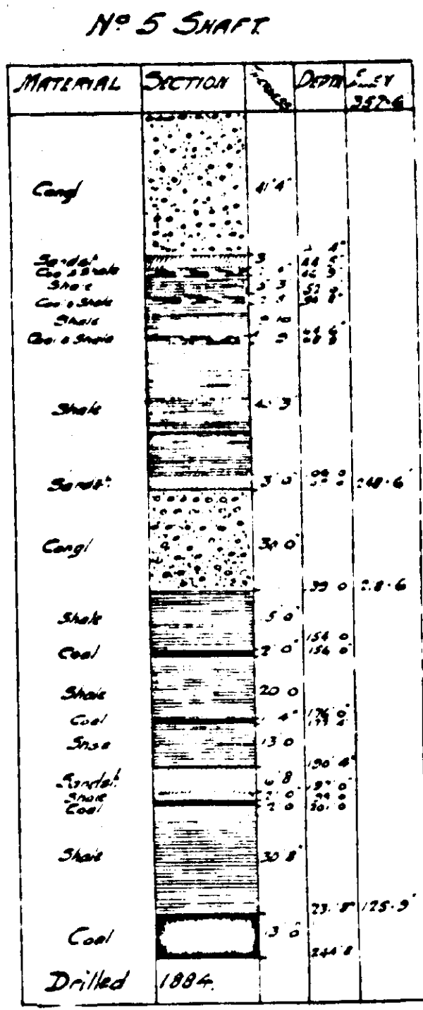
BORE HOLE SECTIONS Scale: 1" = 40'
