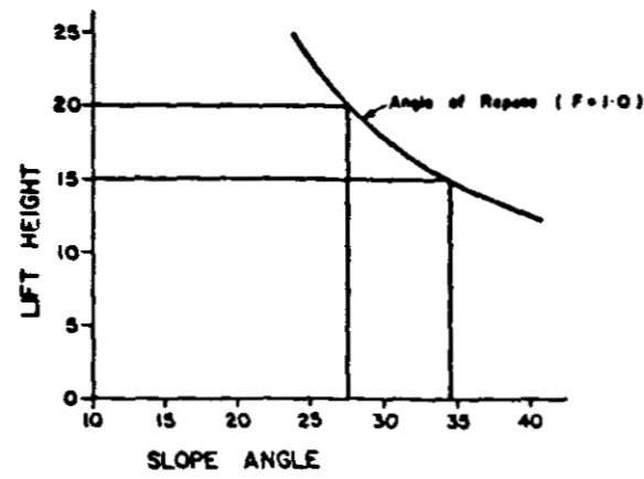
(a) WASTE MATERIAL ANGLE OF REPOSE
