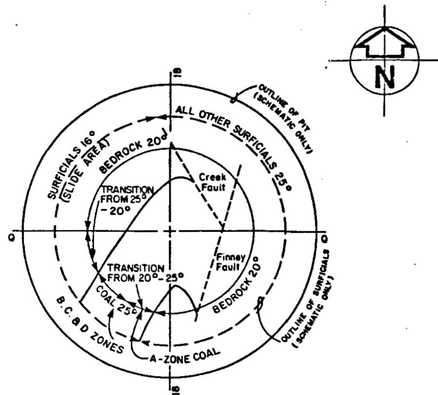
35 YEAR PIT SLOPE ANGLES
