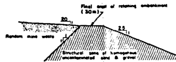
WASTE EMBANKMENT SLOPE ANGLES
