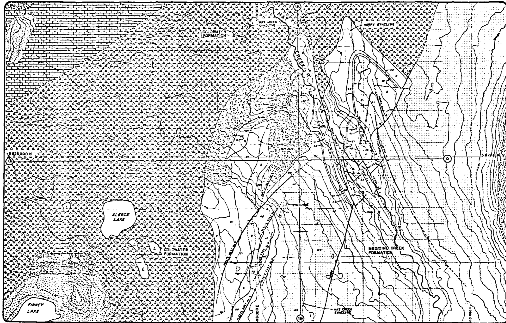
FIGURE 4-2 REGIONAL BEDROCK GEOLOGY NO. 1 DEPOSIT
