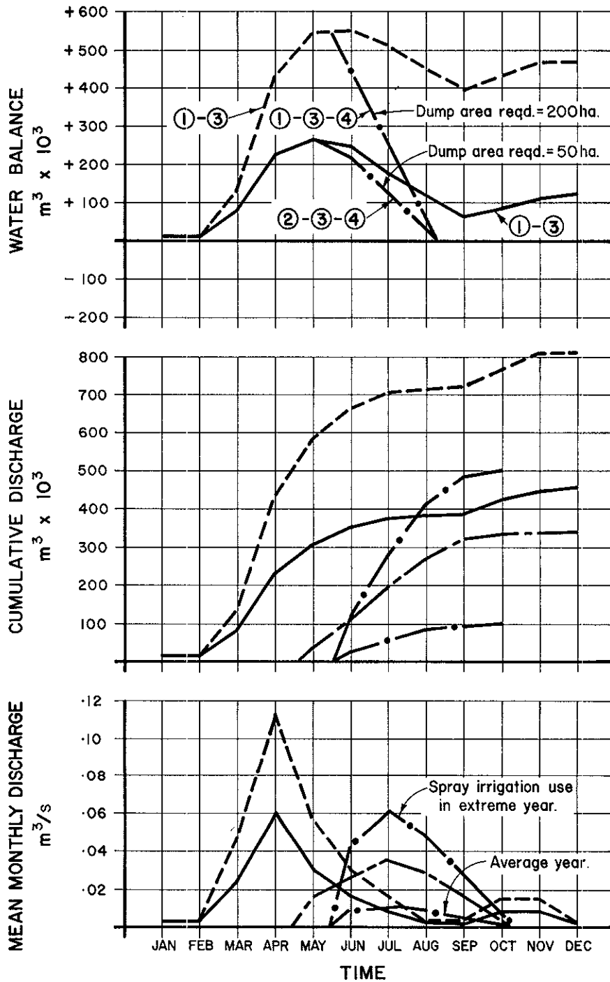
FIGURE 6 - 5 BRITISH COLUMBIA HYDRO & POWER AUTHORITY HAT CREEK PROJECT MINING FEASIBILITY REPORT ZERO DISCHARGE SYSTEM HYDROGRAPHS-YEAR 35
