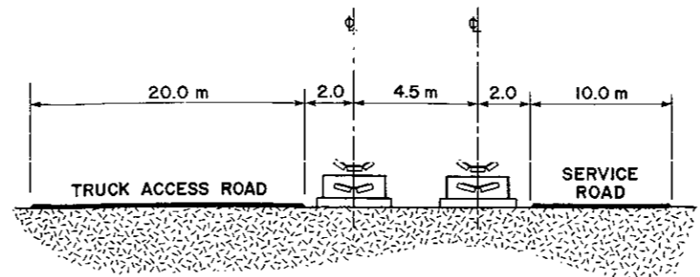
TYPICAL SECTION OVERLAND CONVEYORS
