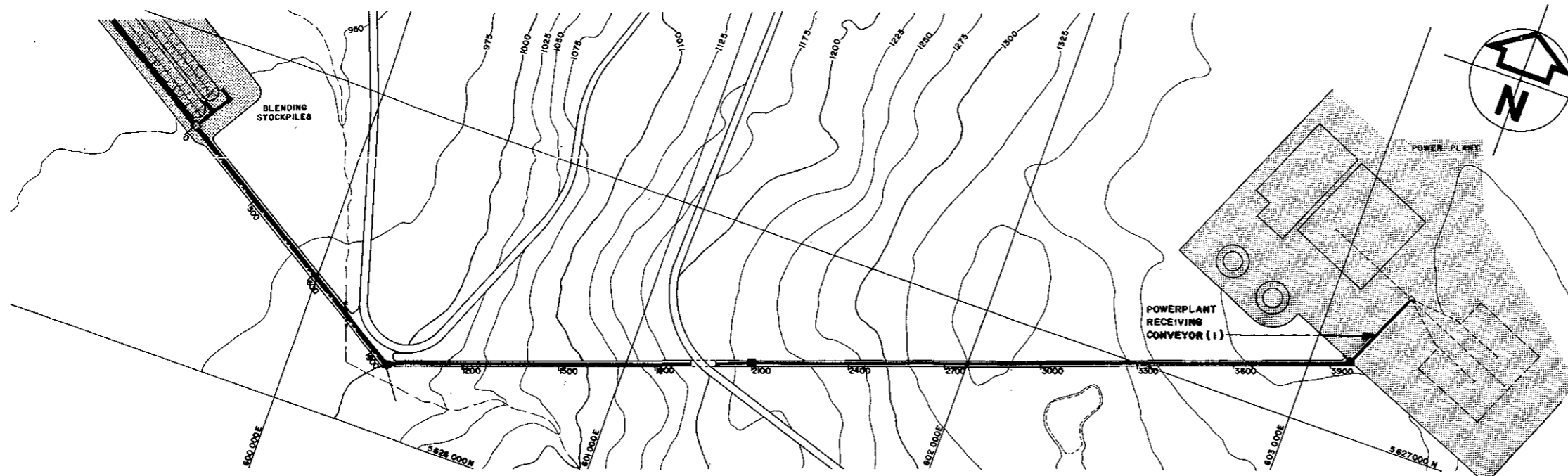
PLAN - OVERLAND COAL CONVEYOR
