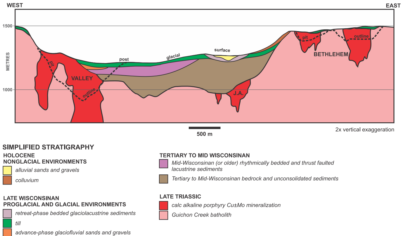
Fig.11. Composite cross-section through Valley, J.A., and Bethlehem porphyry centres showing generalized bedrock topography and simplified cover stratigraphy (see Fig. 3 for porphyry centre locations). Subglacial till samples were collected at surface from the Late Wisconsinan till unit. Units underlying these tills protected bedrock subcrop from glacial erosion during the Late Wisconsinan. These protected bedrock subcrops therefore did not contribute to the geochemical or mineralogical composition of sampled subglacial tills. Simplified stratigraphy modified after Bobrowsky et al. (1993), Byrne et al. (2013), and Plouffe and Ferbey (2015b).
