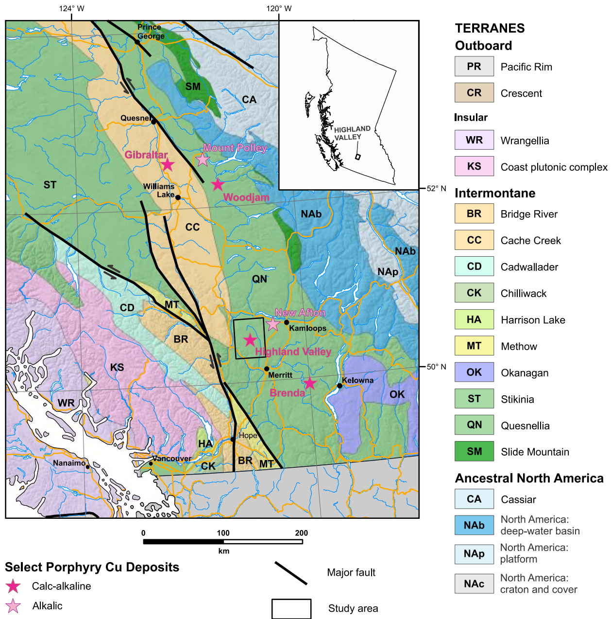
Fig. 1. Study area location. Terranes of the southern Canadian Cordillera after Nelson et al. (2013).
