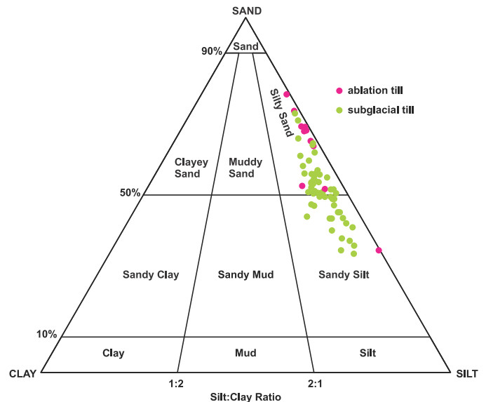
Fig. 8. Grain size analyses of matrix in subglacial (n=55) and ablation (n=11) till samples showing percentage of sand (2 to >0.063 mm), silt (0.063 to >0.002 mm) and clay (<0.002 mm). Classification follows Folk (1954). See Appendix 5.
