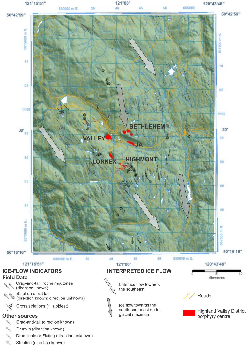
Fig. 4. Ice-flow indicators of Highland Valley Copper mine area. Interpreted ice-flow directions are generalized from data points shown, taking into account topography and expected thickness of Cordilleran ice sheet during full-glacial and late-glacial conditions. Field data from Plouffe and Ferbey (2015a), other sources from Ferbey et al. (2013).
