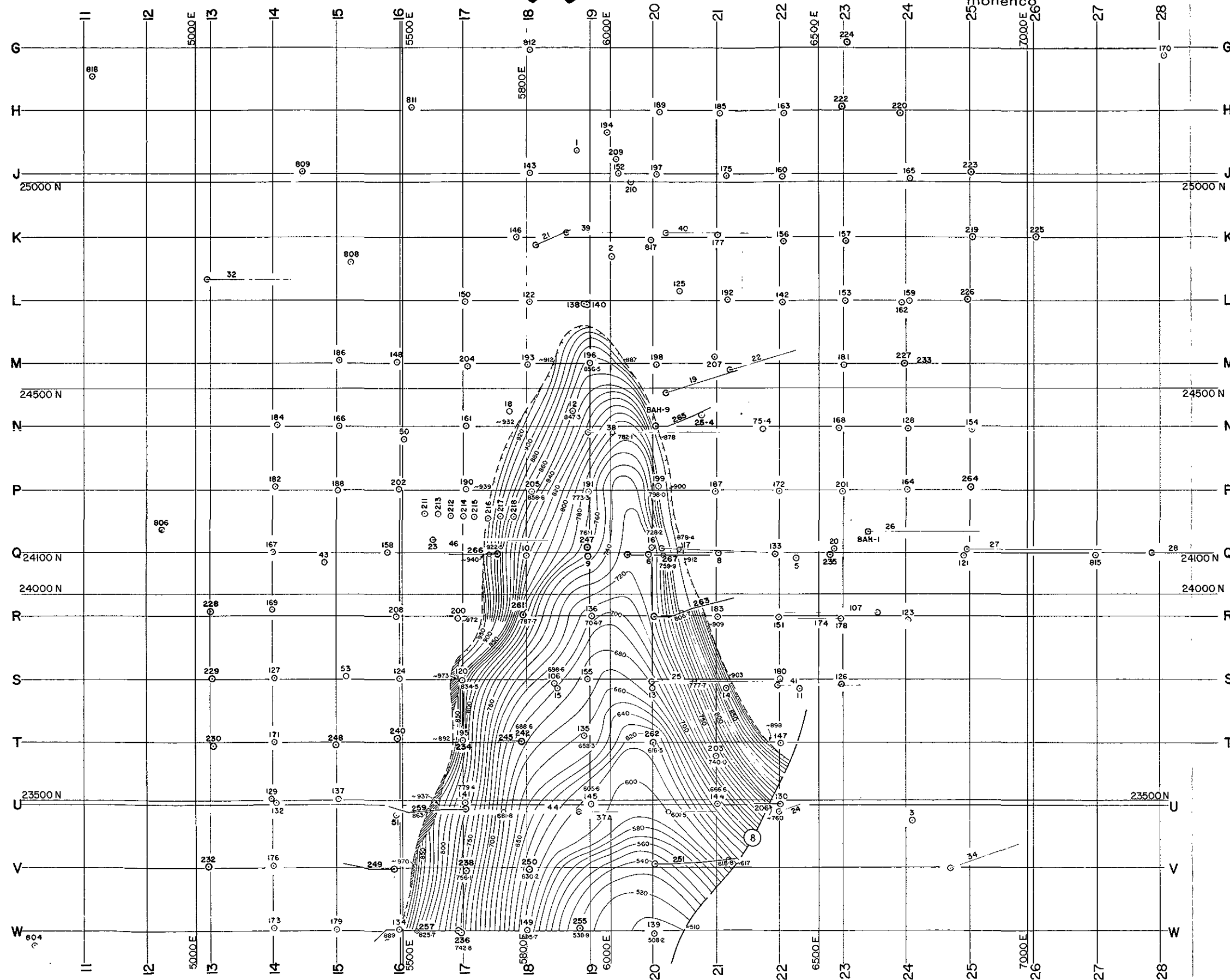
FIGURE 2-11 BRITISH COLUMBIA HYDRO AND POWER AUTHORITY HAT CREEK PROJECT MINING FEASIBILITY REPORT CONTOURS OF TOP OF A-2-1 SUB - ZONE
