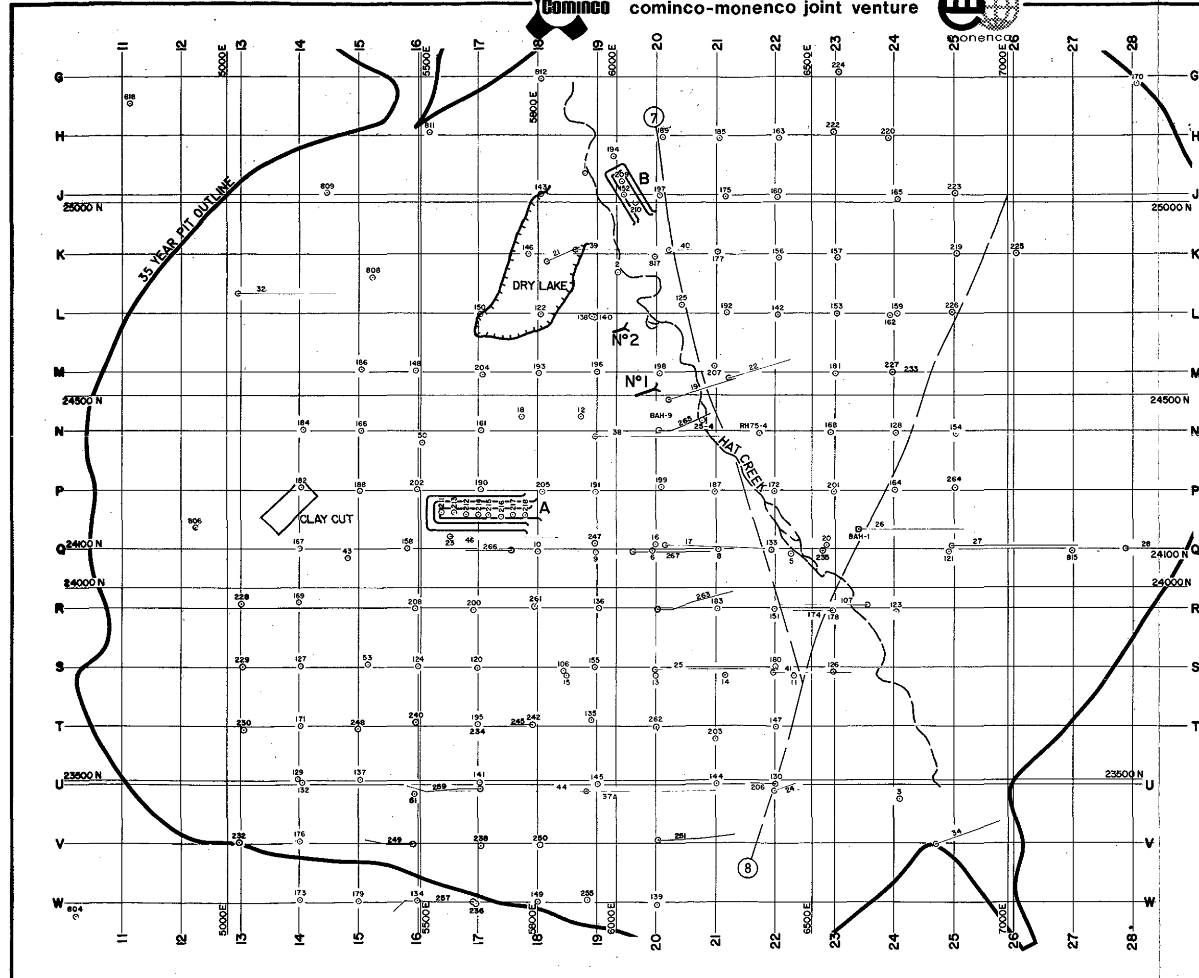
FIGURE 1 - 1 BRITISH COLUMBIA HYDRO AND POWER AUTHORITY HAT CREEK PROJECT MINING FEASIBILITY REPORT DRILLHOLE LOCATION PLAN
