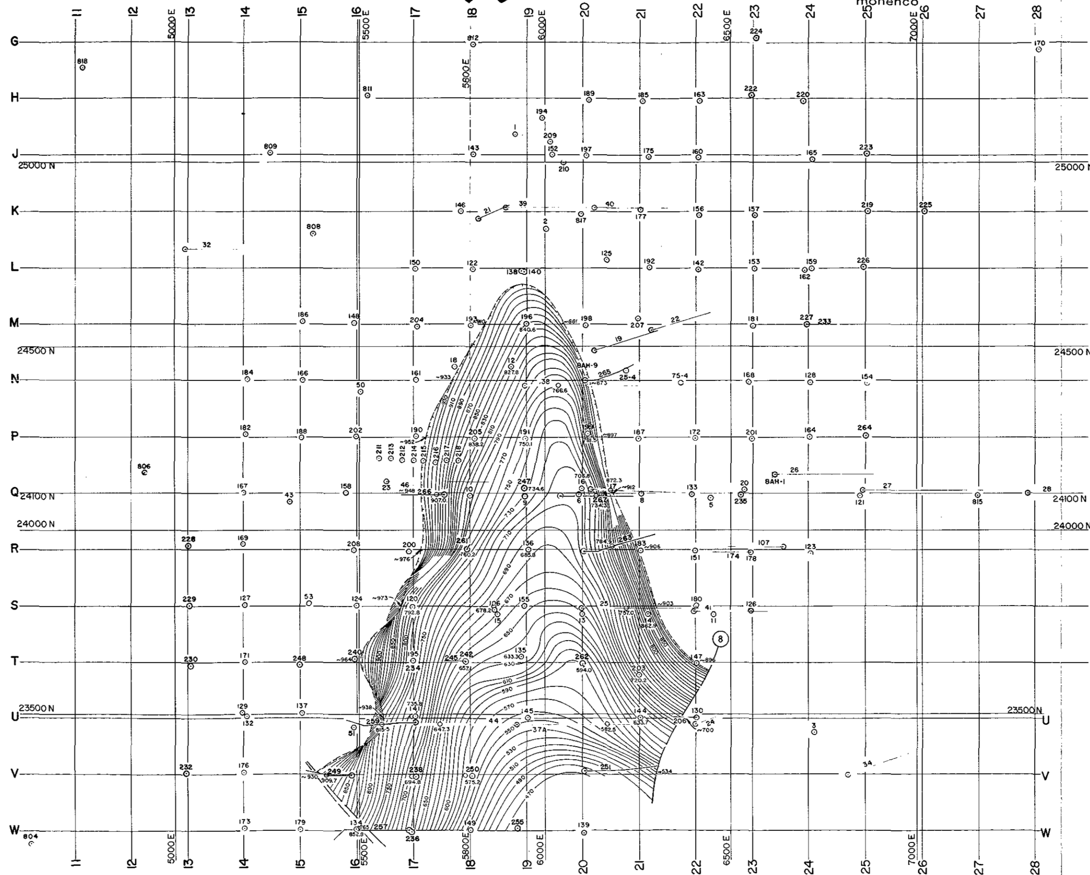
FIGURE 2-12 BRITISH COLUMBIA HYDRO AND POWER AUTHORITY HAT CREEK PROJECT MINING FEASIBILITY REPORT CONTOURS OF TOP OF B-1-1 SUB - ZONE
