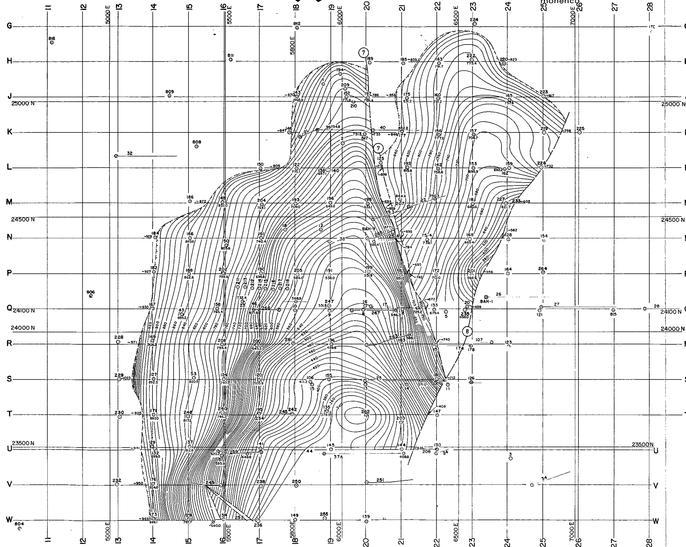
FIGURE 2-13 BRITISH COLUMBIA HYDRO AND POWER AUTHORITY HAT CREEK PROJECT MINING FEASIBILITY REPORT CONTOURS OF BASE OF D-1-4 SUB-ZONE (BASE OF D ZONE)
