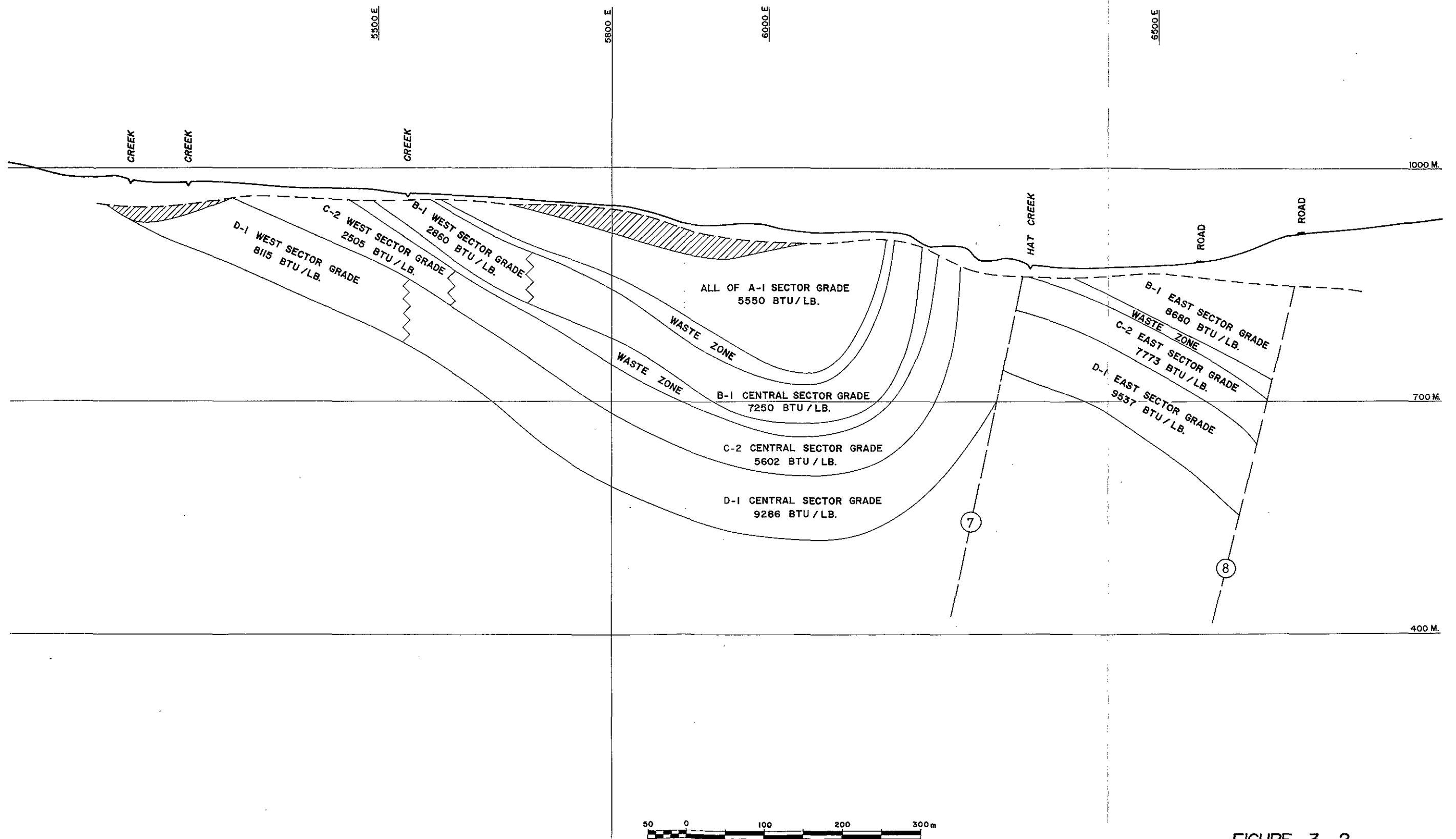
FIGURE 3-2 BRITISH COLUMBIA HYDRO AND POWER AUTHORITY HAT CREEK PROJECT MINING FEASIBILITY REPORT PRELIMINARY COAL QUALITY SECTORS
