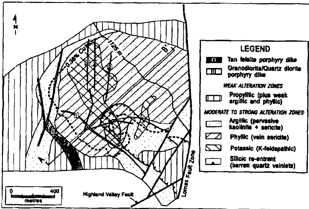
FIGURE 17a. Plan view showing the distribution of major alteration types in the Valley deposit projected to 1125 m level (modified after Ostrenko and Jones, 1976).
