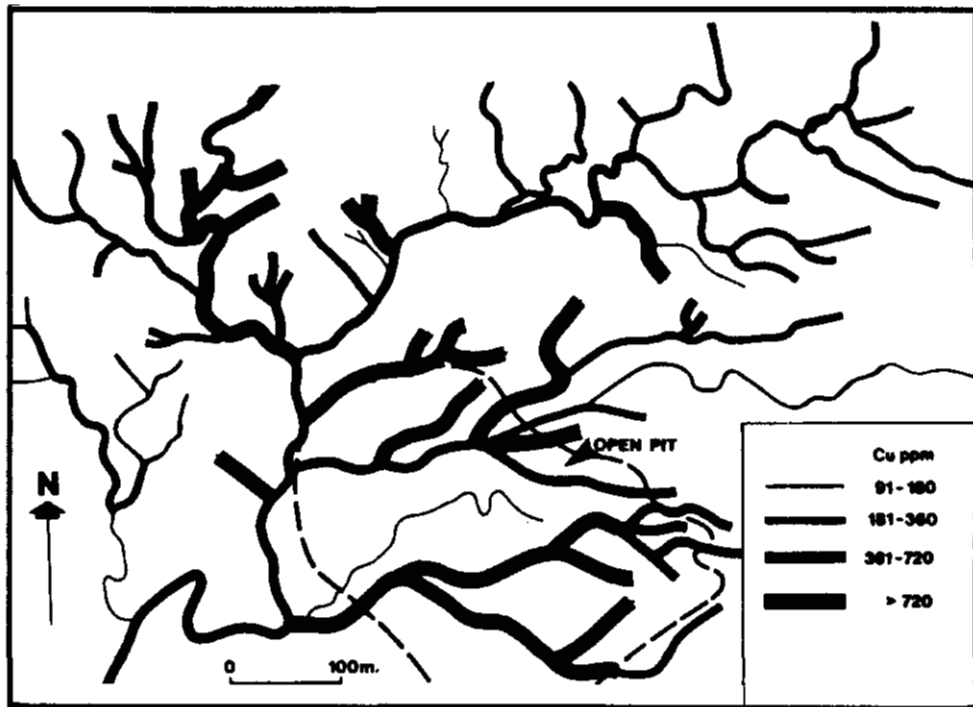
Distribution of copper in stream sediments, Panguna area, Bougainville Island
