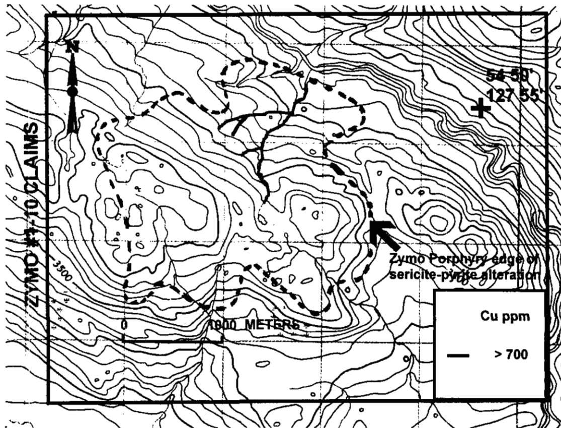
Distribution of copper in stream sediments, Zymo property, B.C.
