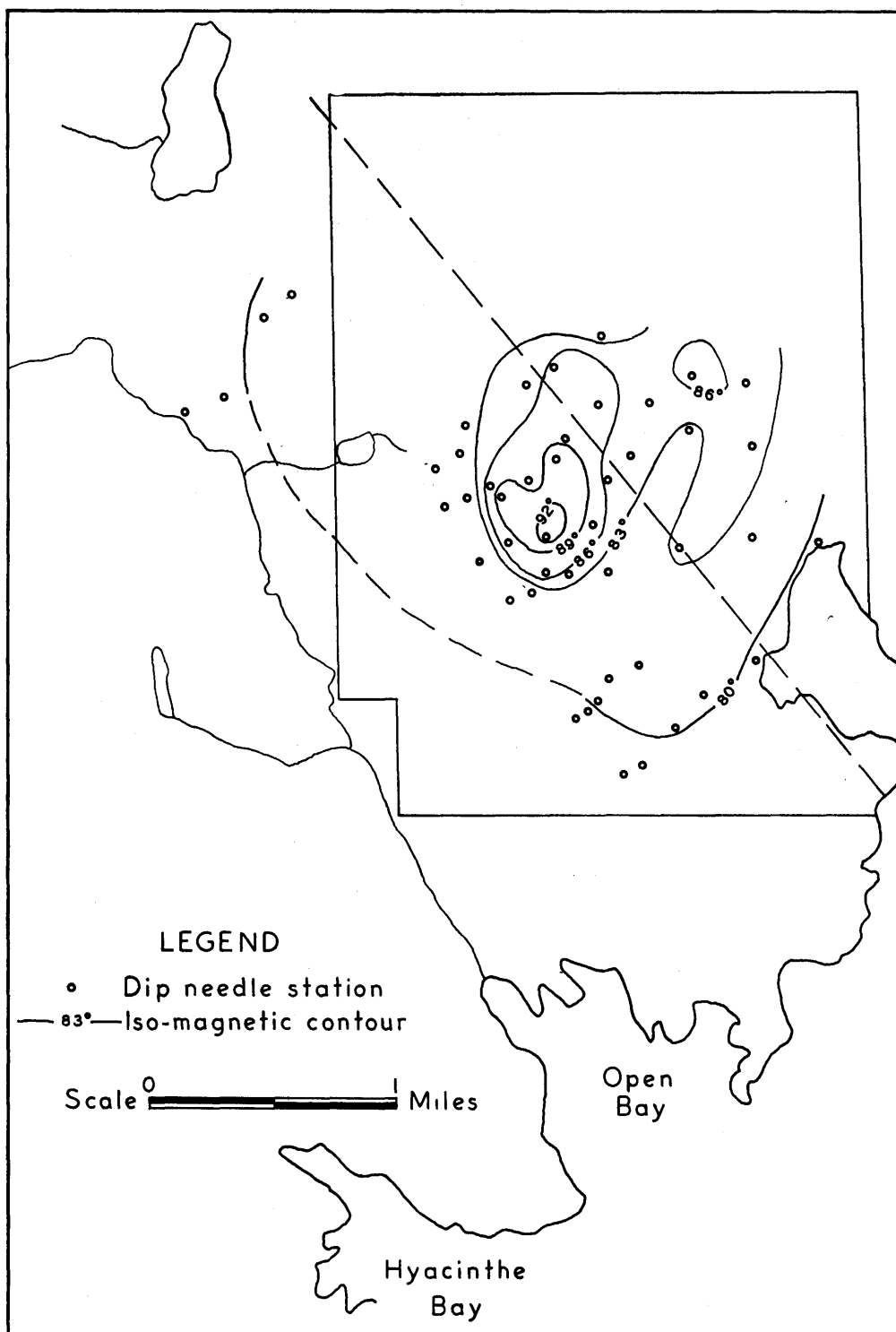
Figure 8.—Dip-needle survey, Quadra Island.
