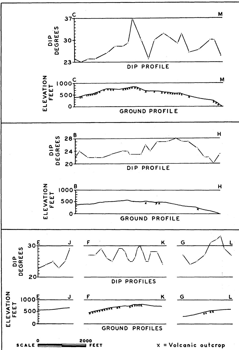
Figure 13A.—Dip-needle and ground profiles, Comet Mountain-Pocahontas Mountain area, Texada Island.
