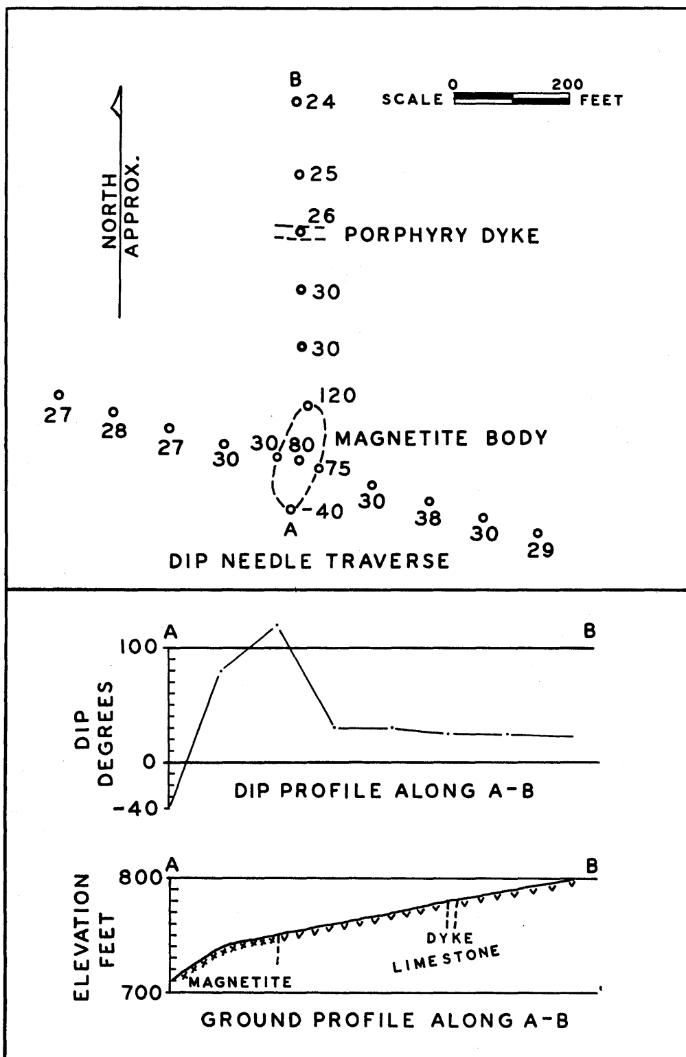
Figure 12.—Dip-needle survey at Cameron orebody, Texada Island.
