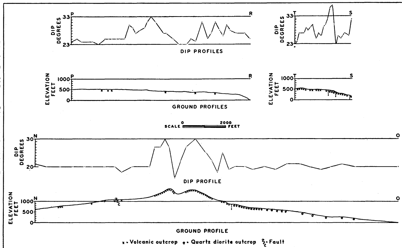
Figure 13B.—Dip-needle and ground profiles, Comet Mountain-Pocahontas Mountain area, Texada Island.
