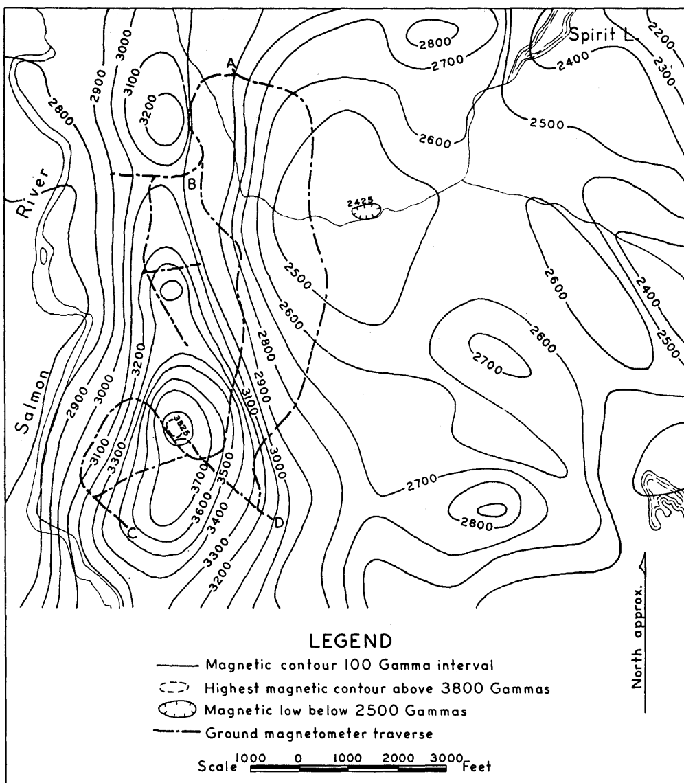
Figure 5.—Aeromagnetic map, Spirit Lake area.
