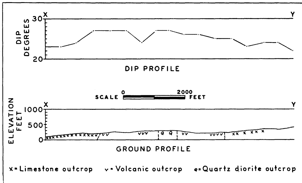
Figure 11.—Dip-needle survey, Priest Lake, Texada Island.
