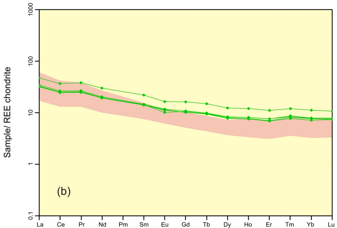
Figure 12. Chondrite-normalized rare earth element plots for diorites from the Boundary Project area, southern British Columbia (normalizing values after Nakamura, 1974): a) diorites from the McKinney Creek area; 07NMA05-15 is tholeiitic in composition, 07NMA05-16 is calcalkaline; b) diorites from the Beaverdell area; pink-shaded field is for all Triassic to Middle Jurassic granodiorites, except for the Mount Baldy stock (Figure 13).
