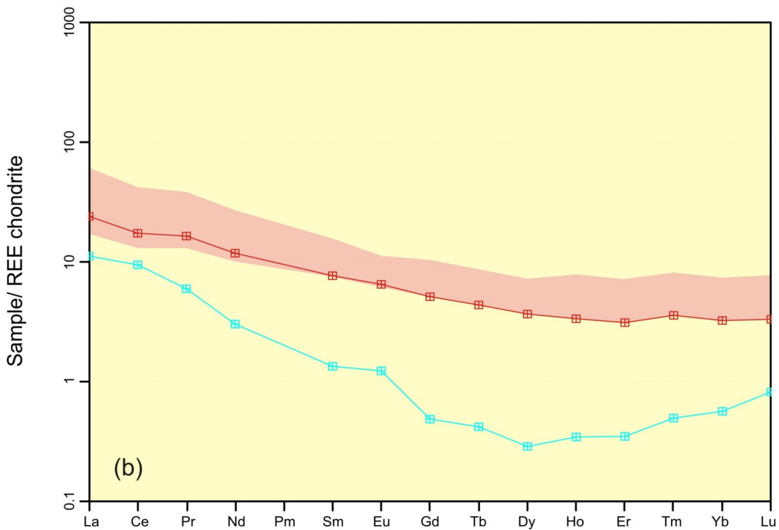
Figure 14. Chondrite-normalized rare earth element plot for rocks in the Boundary Project area, southern British Columbia: a) Tertiary granitic McKinney Creek stock (solid blue squares) and Beaverdell suite stocks (blue crosses; normalizing values after Nakamura, 1974); 07NMA28-17 is the alkalic Collier Creek stock and 07NMA38-01 an unnamed stock west of Crouse Creek. b) Early Jurassic Ed James Creek biotite-feldspar-quartz orthogneiss (red crossed squares) and undated, unfoliated leucogranite (blue crossed squares). For comparison, the pink-shaded field is for the Triassic to Middle Jurassic granodiorite, except the Mount Baldy stock (Figure 13).
