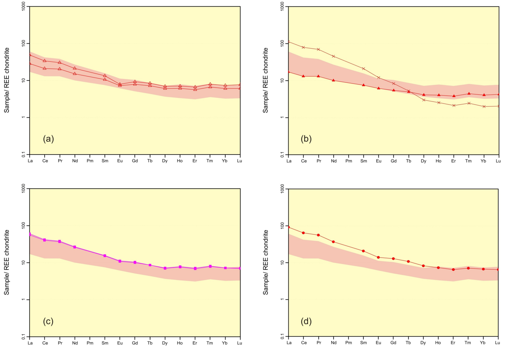
Figure 13. Chondrite-normalized rare earth element plots for Triassic and Jurassic granitic rocks in the Boundary Project area, southern British Columbia (normalizing values from Nakamura, 1974): a) Triassic West Kettle batholith; b) Middle Jurassic Greenwood stock (closed red triangles) and Mount Baldy stock (red Xs); c) Middle Jurassic Gidon Creek stock; d) Late Jurassic Myers Creek stock. For comparison, the pink-shaded field in all diagrams includes all Triassic to Middle Jurassic intrusions except the Mount Baldy stock.
