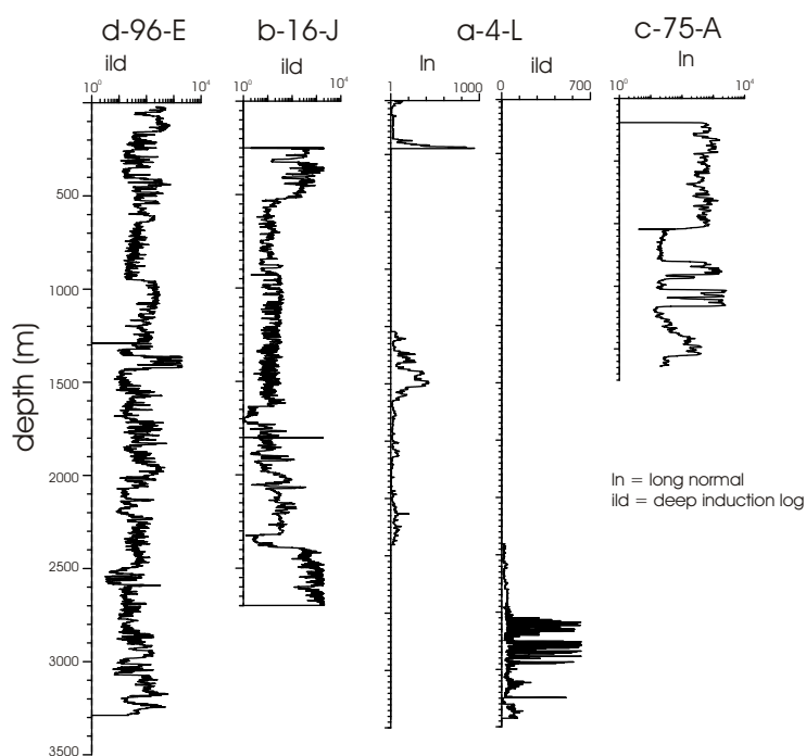
Figure 4. Resistivity data measured at four of the wells in the southern Nechako region.
